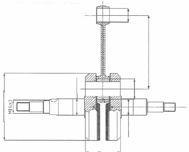
Ny veivaksel (2007 mod.)
