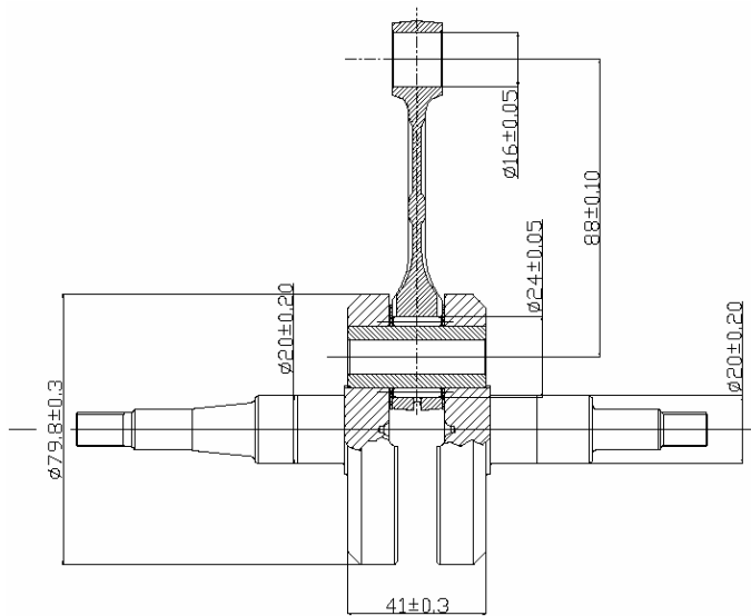
Gammel veivaksel (2006 mod.)
