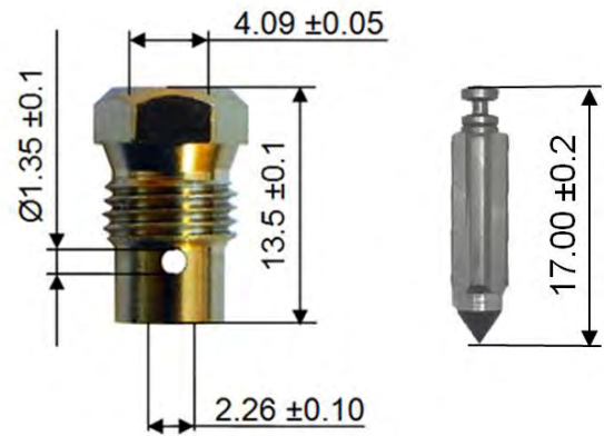
REF.37/1 - P. N° 233-721P SEAT + NEEDLE
