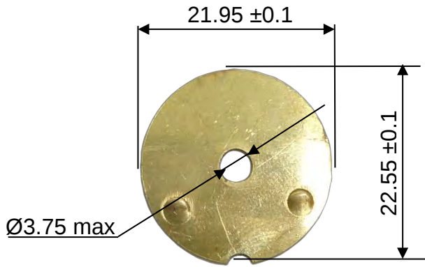
REF.33 - P. N° 14-A96 THROTTLE SHUTTER
